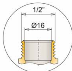
Art. 1668 (1/2") per tubi multistrato for multilayer pipe Ø14x2,0 Ø16x2,0 Ø18x2,0 Ø20x2,0
